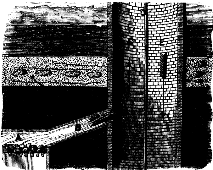
Fig. 43. A. Furnace. B. The furnace drift. C. The up-cast shaft. D. The brattice, or timber partition separating the up-cast from E, the down-cast, from which the air travels to the various galleries of the pit, passing to the furnace A B, and so to the up-cast C.
